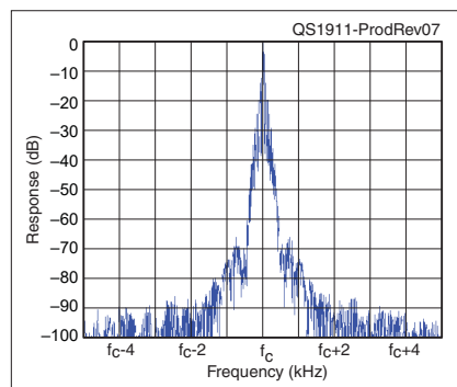
Figure 7 — Spectral display of the Yaesu FTDX101D transmitter during keying sideband testing. Equivalent keying speed is 60 WPM using external keying and the default rise time setting. Spectrum analyzer resolution bandwidth is 10 Hz, and the sweep time is 30 seconds. The transmitter was being operated at 100 W PEP output on the 14 MHz band, and this plot shows the transmitter output \pm 5 kHz from the carrier. The reference level is 0 dBc, and the vertical scale is in decibels.
