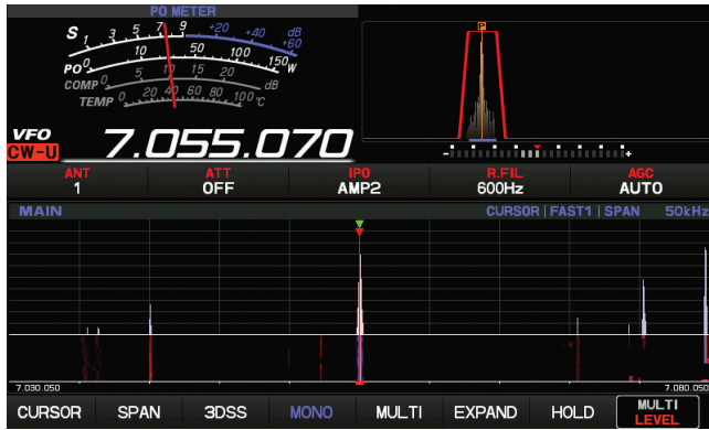
Figure 1 — The Yaesu FTDX101D display showing a single waterfall view for 50 kHz of the 40-meter band centered on the frequency tuned by VFO A. The “filter function display” at the upper right shows the received passband with the received signal within. The spectrum span can be adjusted from a width of 1 kHz to 1 MHz in 10 steps.
